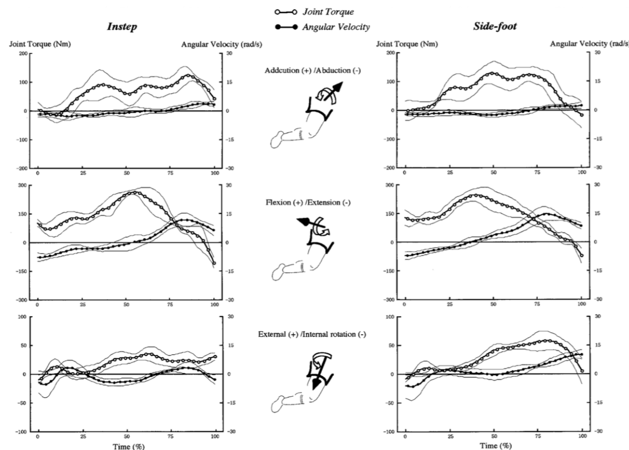
FIGURE 3—Changes in joint torque and angular velocity at the hip of the side-foot (right column) and instep (left column) kicks. For the hip adduction/abduction (top), positive and negative values corresponded to adduction and abduction, respectively. For the hip flexion/extension (middle), positive and negative values corresponded to flexion and extension, respectively. For the hip external/internal rotation (bottom), positive and negative values corresponded to external and internal rotation, respectively.
